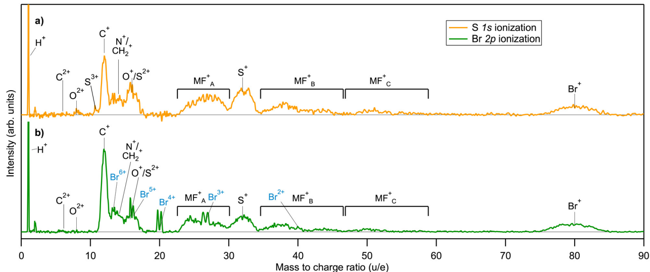
Fig. 4 Ion mass spectra of BrSDU measured in coincidence with the S 1s (a) and Br 2p_{3/2} (b) photoelectrons, normalized by the height of the \text{Br}^+ peaks. In addition to the labeled atomic ions, the mass-ranges of significant molecular fragments are marked by \text{MF}_{A,B,C}^+ and \text{CH}_2^+ . Sharp doublet features \text{Br}^{3+} – \text{Br}^{6+} are assigned to contaminant HBr.
