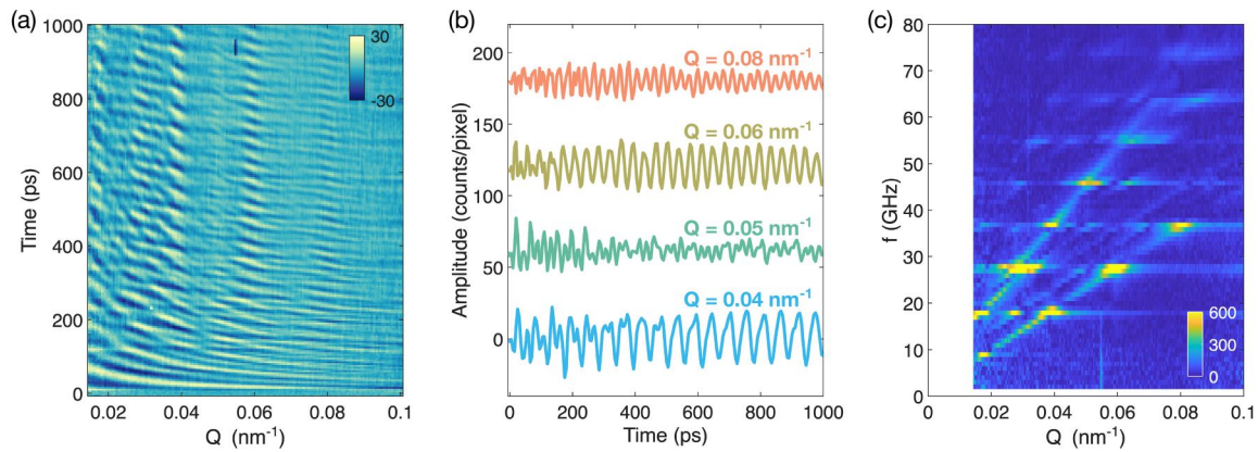
FIG. 2. (a) Azimuthally integrated DES intensity as a function of wavevector Q and pump-probe delay \Delta t , measured in transmission geometry for the 200-nm-Ti/200-nm-SiN sample (color scale: counts per pixel). (b) Time dependence of the DES signal in (a) at selected Q values. (c) Modulus of the temporal Fourier transform of the data in (a), yielding a frequency-wavevector map (color scale: arbitrary units).
