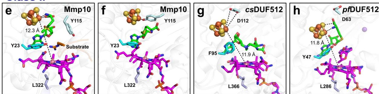
Fig. 9 Structures of the active sites of B 12 -dependent radical SAM enzymes showing the positions of key residues. Close-ups of the active sites of (a) OxsB, (b) TokK, (c) TsrM, (d) QCMT, (e) Mmp10 with and (f) without substrate, (g) csDUF512 and (h) pfDUF512. Residues involved in the tetra coordination of the cluster (E273/TsrM, Y115/Mmp10, D112/csDUF512 and D63/pfDUF512) are shown in pale cyan. Amino acids in the lower axial position of cobalamin (N186-water107/OxsB, W76/TokK, R69/TsrM, L322/Mmp10, L366/csDUF512, L286/pfDUF512) are shown in light blue. Residues between the cobalamin cofactor and the [Fe 4 S 4 ] cluster (W215/TokK, E236/TsrM, Y23/Mmp10, F95/csDUF512, Y47/pfDUF512) are shown in cyan. The cobalamin cofactor is shown in magenta, the [Fe 4 S 4 ] cluster in orange and yellow spheres, and the SAM (SAM cleavage products in TokK, aza-SAM in both TsrM and csDUF512 and SAH in pfDUF512) in green. Substrates are shown in orange. The distance between the cobalt atom of cobalamin and the proximal iron from the [Fe 4 S 4 ] cluster is indicated with a black dashed line. (TokK: PDB 7KDY; OxsB: PDB 5UL4; TsrM: PDB 6WTF; QCMT: PDB 9CCB; Mmp10: PDB 7QBS; csDUF512: PDB 9CG1; pfDUF512: PDB 9CG2).
