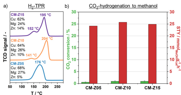
Fig. 1 a) H 2 -TPR profiles (5 K min -1 , 10% H 2 /Ar, 50 mL min -1 ) and b) CO 2 conversion and STY for methanol during CO 2 -hydrogenation (230 °C, H 2 /CO 2 = 3 : 1, 30 bar, WHSV = 75 000 mL g cat -1 h -1 , 1 h hold).
