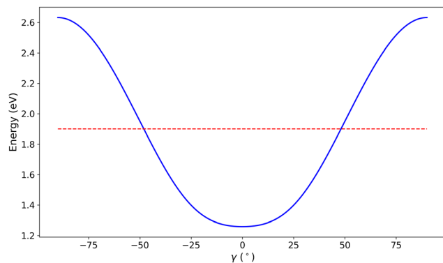
Fig. 6 Potential of the 1A' PES as a function of the Jacobi angle for r = 2.63 bohr and R = 4.14 , corresponding to the position of SP1_{1A'} in the Jacobi coordinates. The QCT threshold energy for which the reaction opens is marked by the red dashed line.
