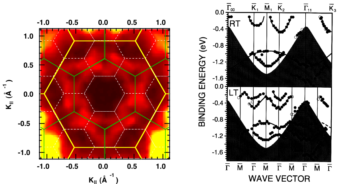
Figure 8 (left panel) Fermi surface of (\sqrt{3}\times\sqrt{3})R30^\circ reconstruction of Pb on Ge at RT and (right panel) experimental band structure of the same phase, PRB 57,14758(1998).
