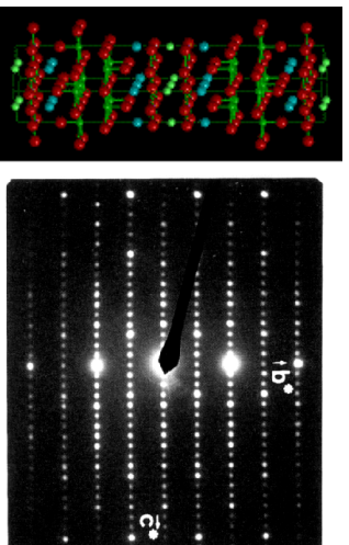
Figure 4. Structure and Diffraction pattern of a Bi2212 crystal. Those samples are the prototypical systems in superconducting materials due to their crystal perfection.
