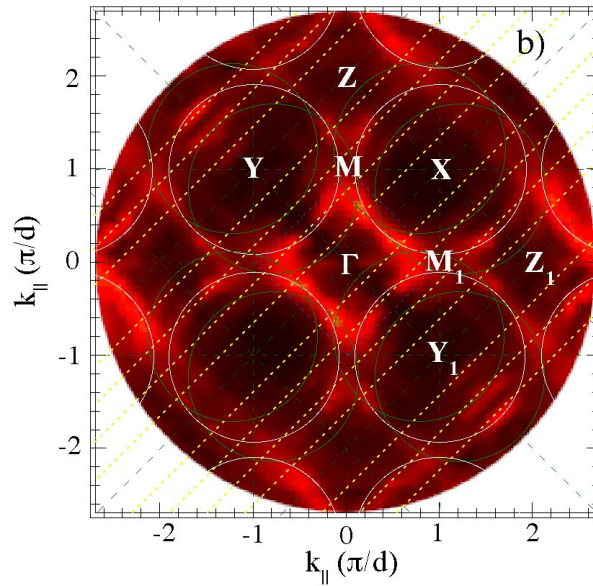
Figure 5. The figure shows large portions of the Fermi surface of a Fermi Surface of \text{Bi}_2\text{Sr}_2\text{CaCuO}_{8+\delta} crystal at the optimum doping with T_c=91 K, (measured at the SU8, September 2000).
